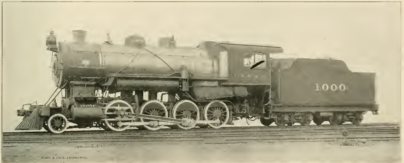
HEAVY CONSOLIDATION ENGINE FOR THE LAKE SHORE.
